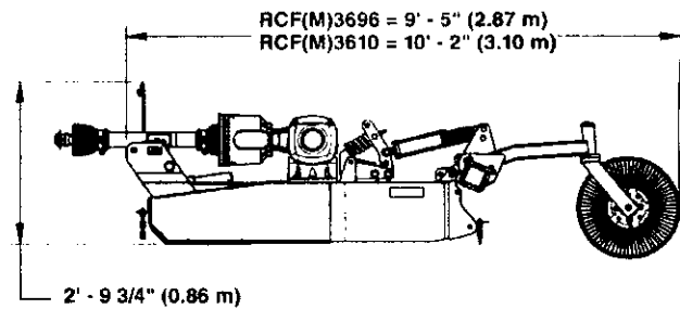
Semi-Mounted Rotary Cutter (RC3696 Shown)
