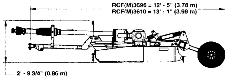
Pull-Type Rotary Cutter (RC3696 Shown)
