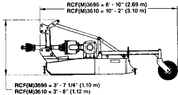
3-Point Mounted Rotary Cutter (RC3696 Shown)
